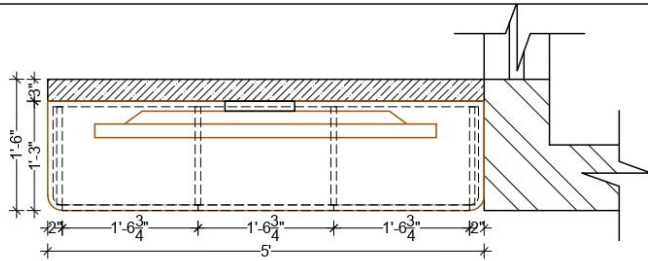
PLAN
