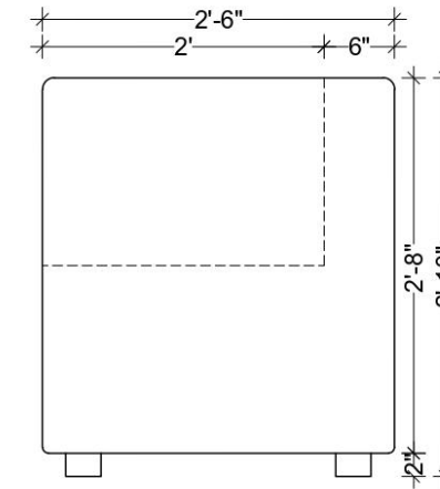
SIDE ELEVATION
