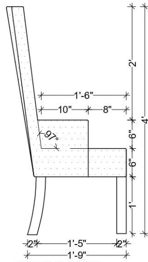
SIDE ELEVATION
