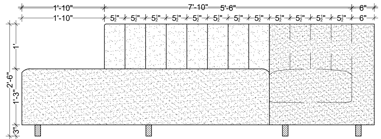
SIDE ELEVATION
