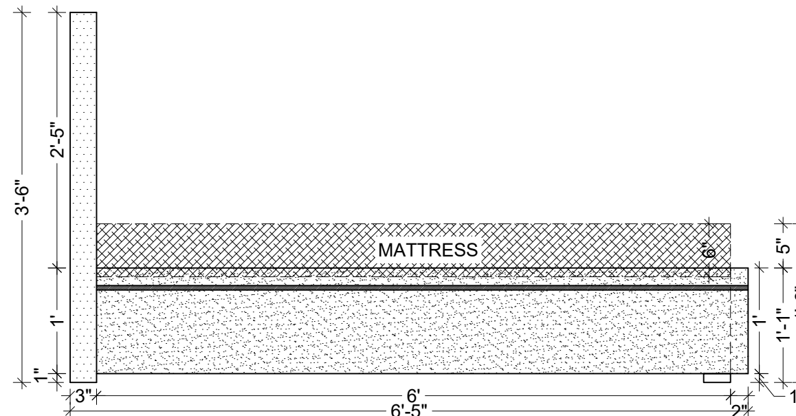
SIDE ELEVATION
