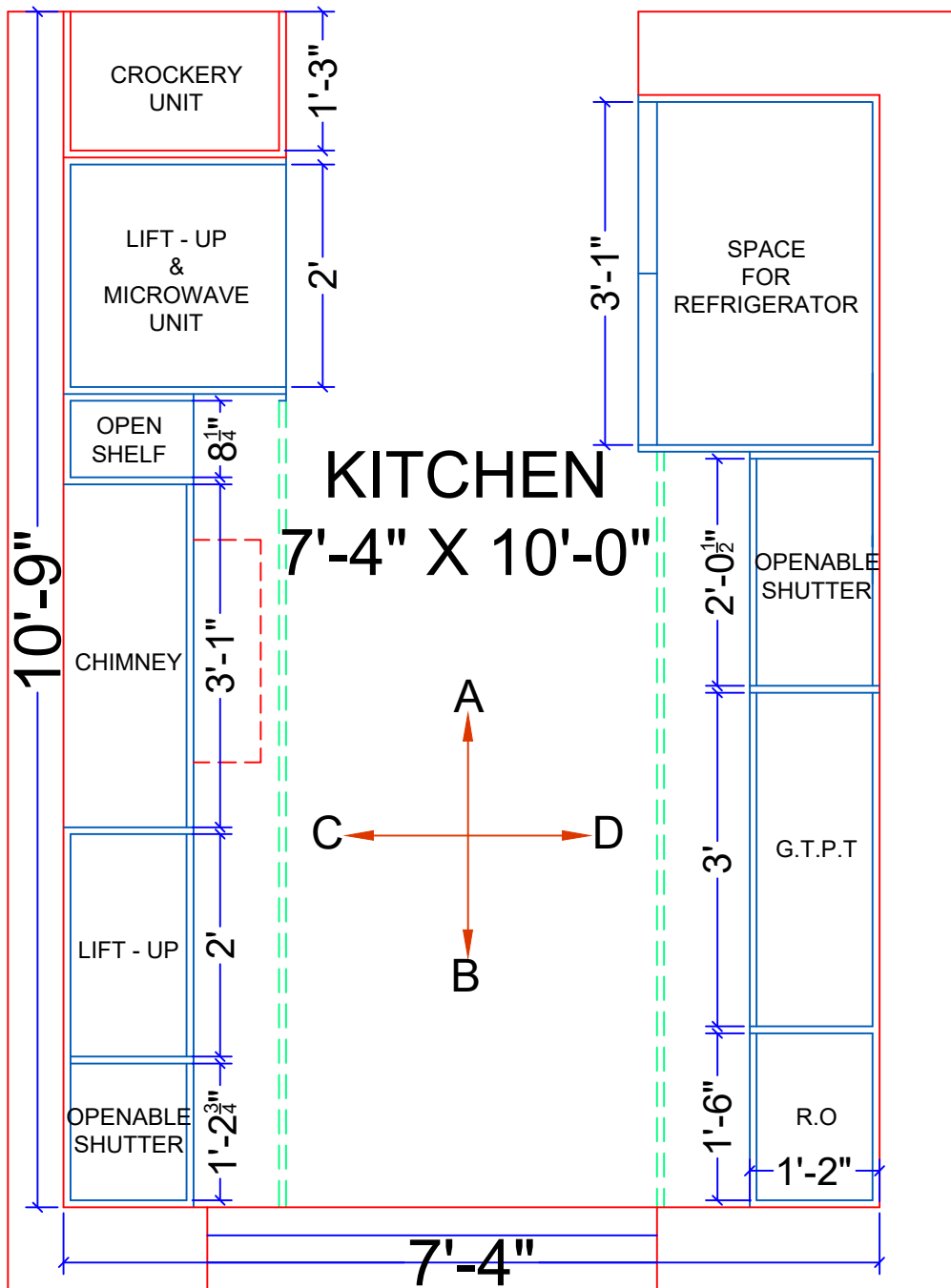
ABOVE COUNTER PLAN
