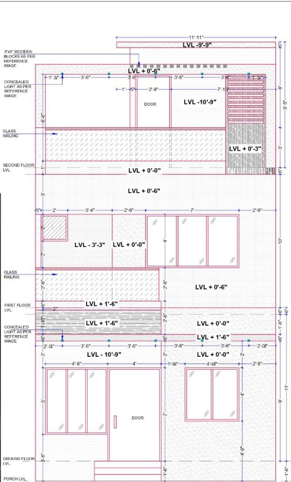
FRONT ELEVATION
