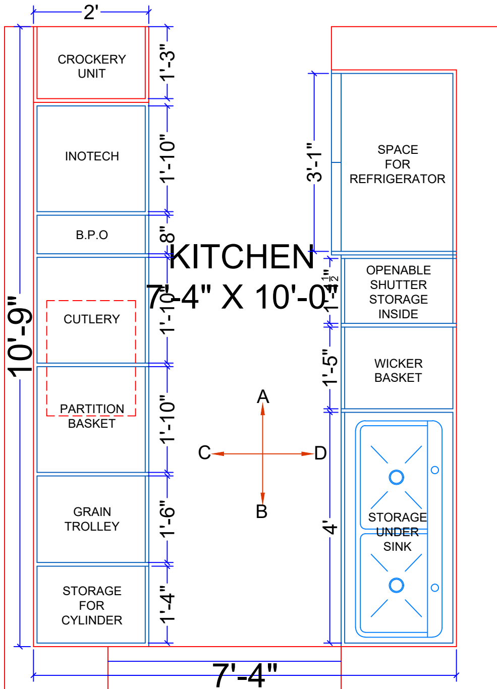
BELOW COUNTER PLAN
