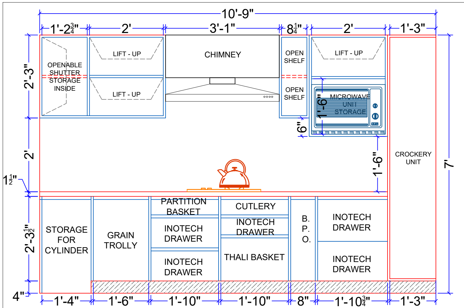
ELEVATION C
